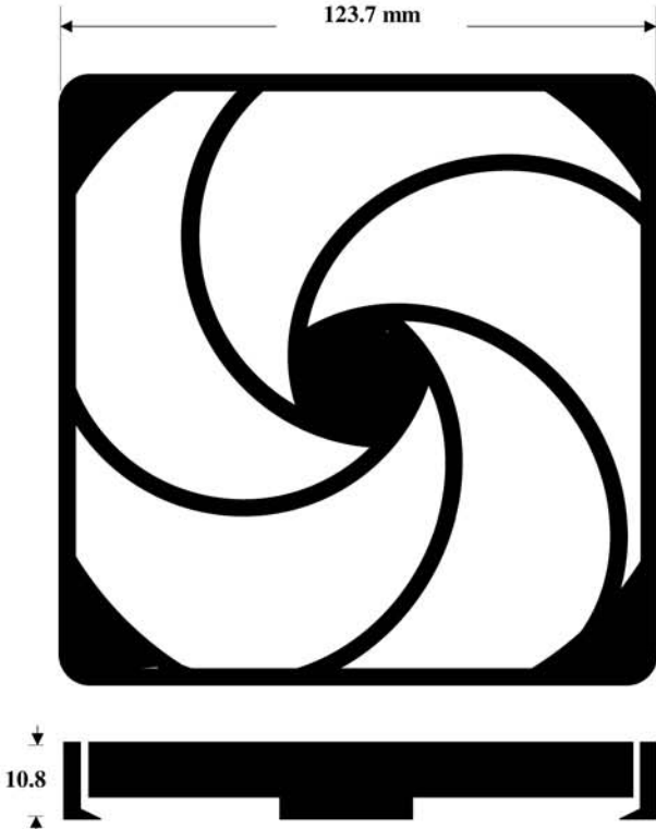
Retainer "R" / R120P
