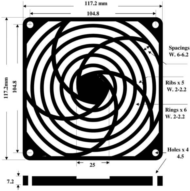
Guard "G" / G120P
