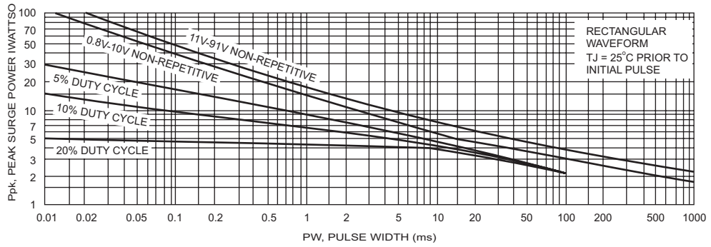
FIG.11- MAXIMUM SURGE POWER
