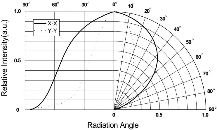
Radiation Characteristics
