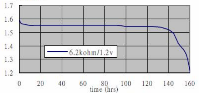
Typical discharge curve at 20\pm 2^\circ\text{C}
