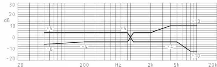
Frequency Response
