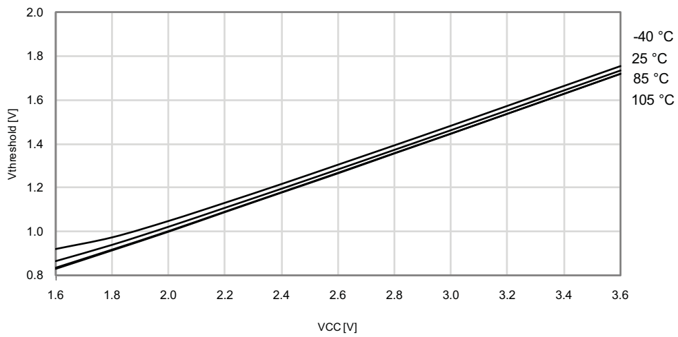
Figure 33-170. I/O Pin Input Threshold Voltage vs. V_{CC}
