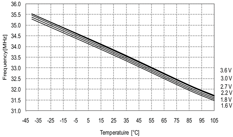
Figure 33-271. 32MHz Internal Oscillator Frequency vs. Temperature DPLL disabled
