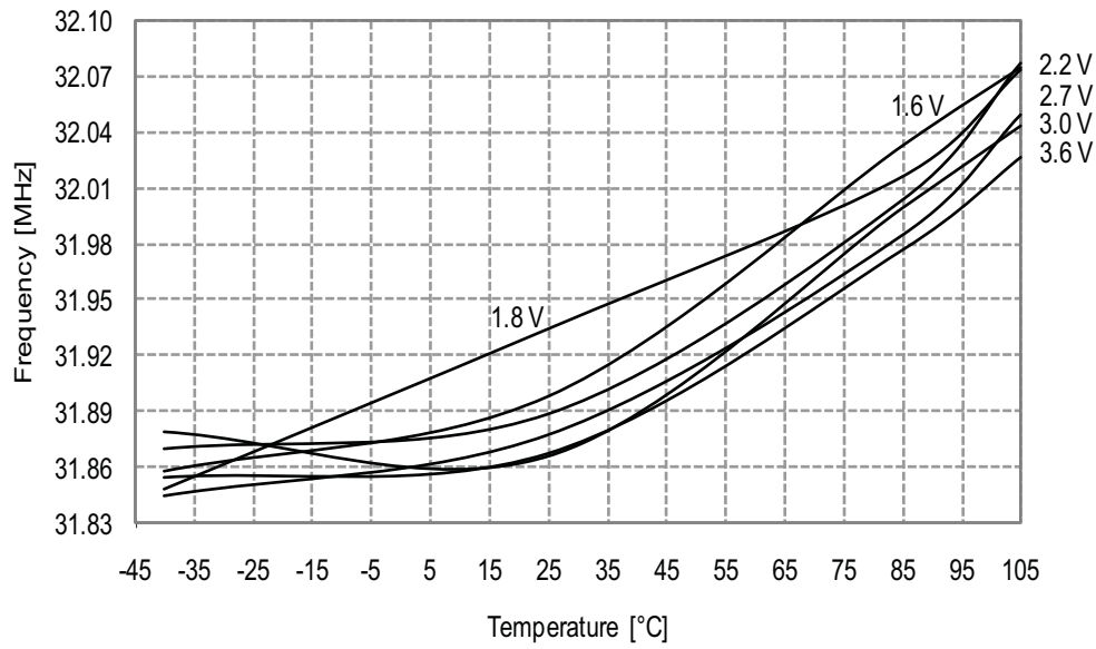
Figure 33-272. 32MHz Internal Oscillator Frequency vs. Temperature DPLL enabled, from the 32.768kHz internal oscillator
