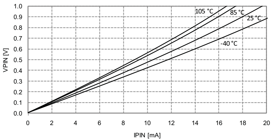
Figure 33-308. I/O Pin Output Voltage vs. Sink Current
