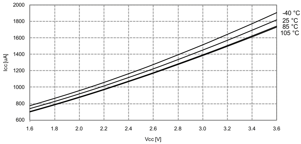
Figure 33-255. Idle mode supply current vs. V_{CC} .
