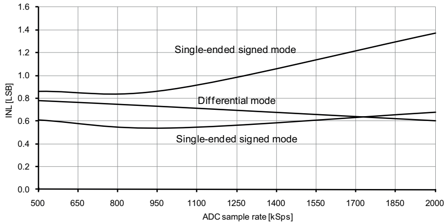
Figure 33-195. INL error vs. sample rate. T = 25°C, V CC = 2.7V, V REF = 1.0V external.
