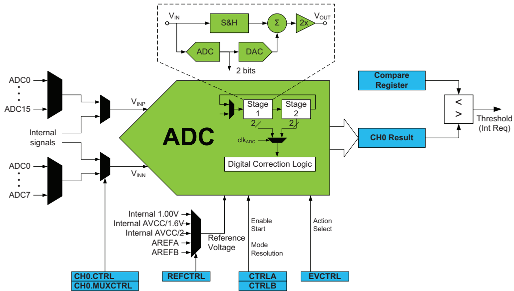
Figure 25-1. ADC overview.
