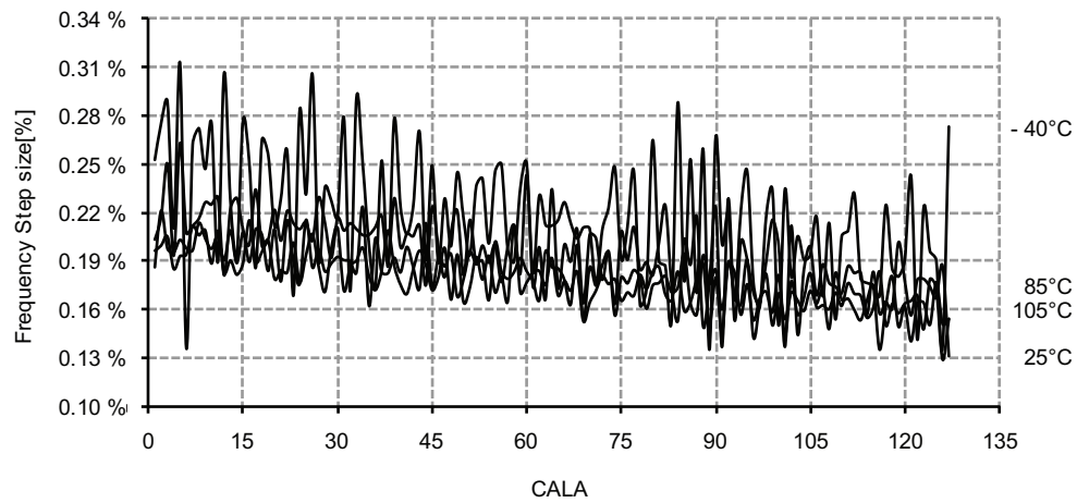
Figure 33-236. 32MHz internal oscillator CALA calibration step size.
