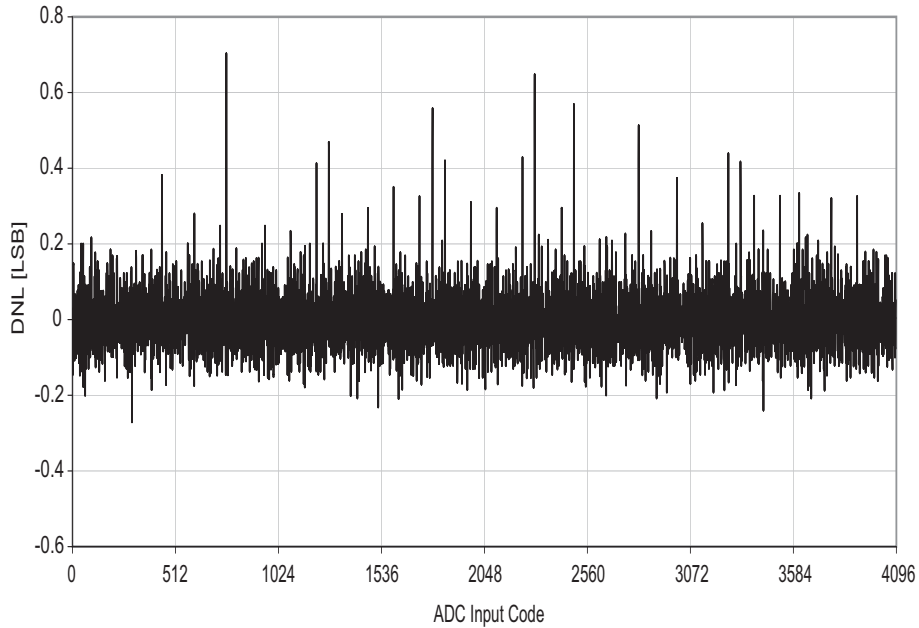
Figure 33-283. DNL error vs. input code
