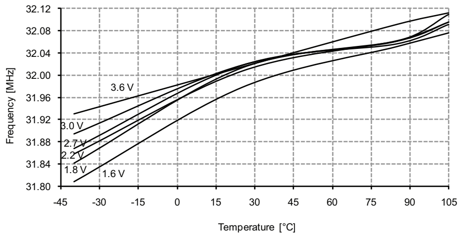
Figure 33-235. 32MHz internal oscillator frequency vs. temperature.
