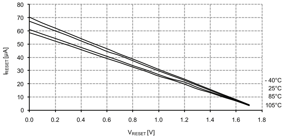
Figure 33-221. Reset pin pull-up resistor current vs. reset pin voltage.
