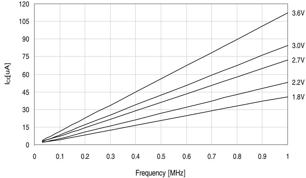
Figure 33-87. Idle mode supply current vs. frequency.
