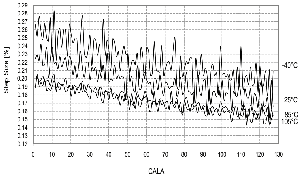
Figure 33-149. 2MHz internal oscillator CALA calibration step size.
