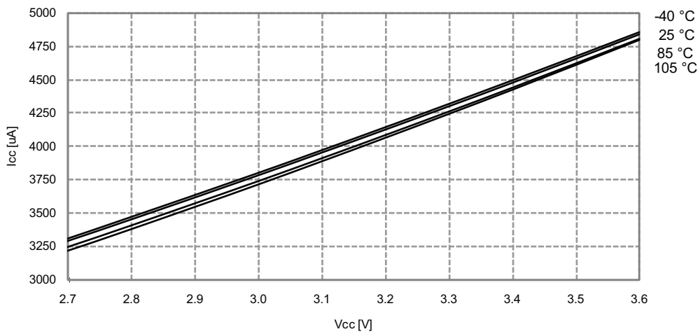
Figure 33-256. Idle mode current vs. V_{CC} .
