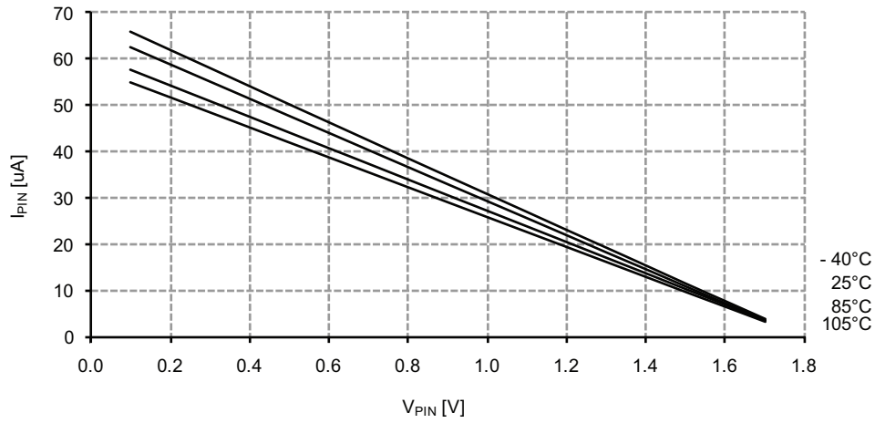
Figure 33-179. I/O pin pull-up resistor current vs. input voltage.
