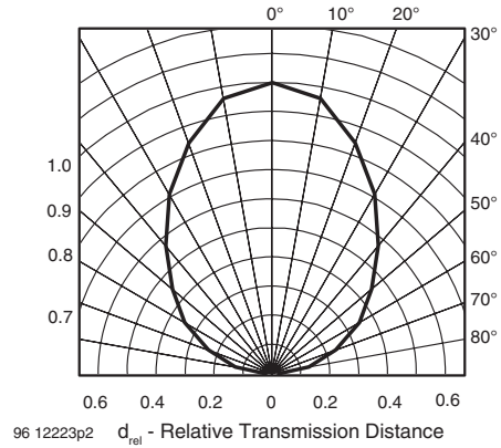
Fig. 12 - Horizontal Directivity
