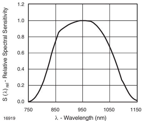
Fig. 11 - Relative Spectral Sensitivity vs. Wavelength
