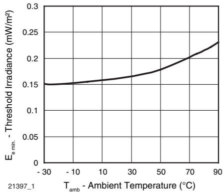
Fig. 10 - Sensitivity vs. Ambient Temperature
