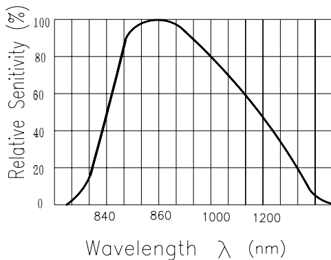
Fig.5 Spectral Sensitivity
