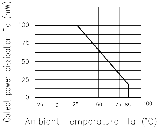
Fig.1 Collector Power Dissipation vs. Ambient Temperature
