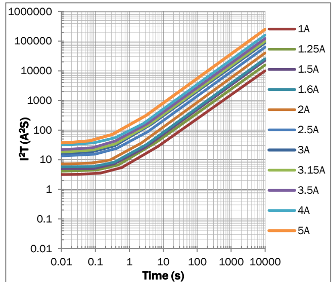
I 2 T vs Time Curve
