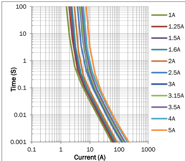
Time-Current Curve
