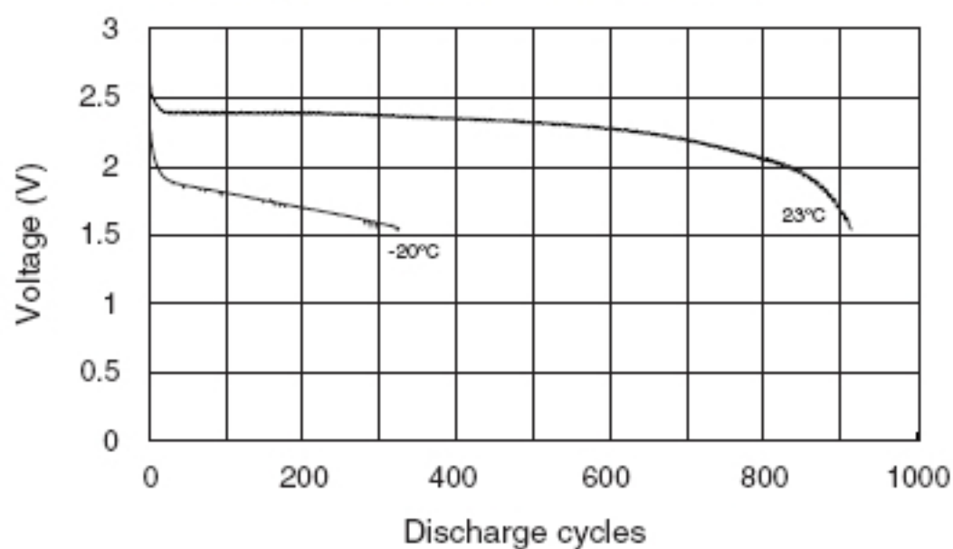
Discharge Characteristics 900mA, 3 seconds on / 27 seconds off
