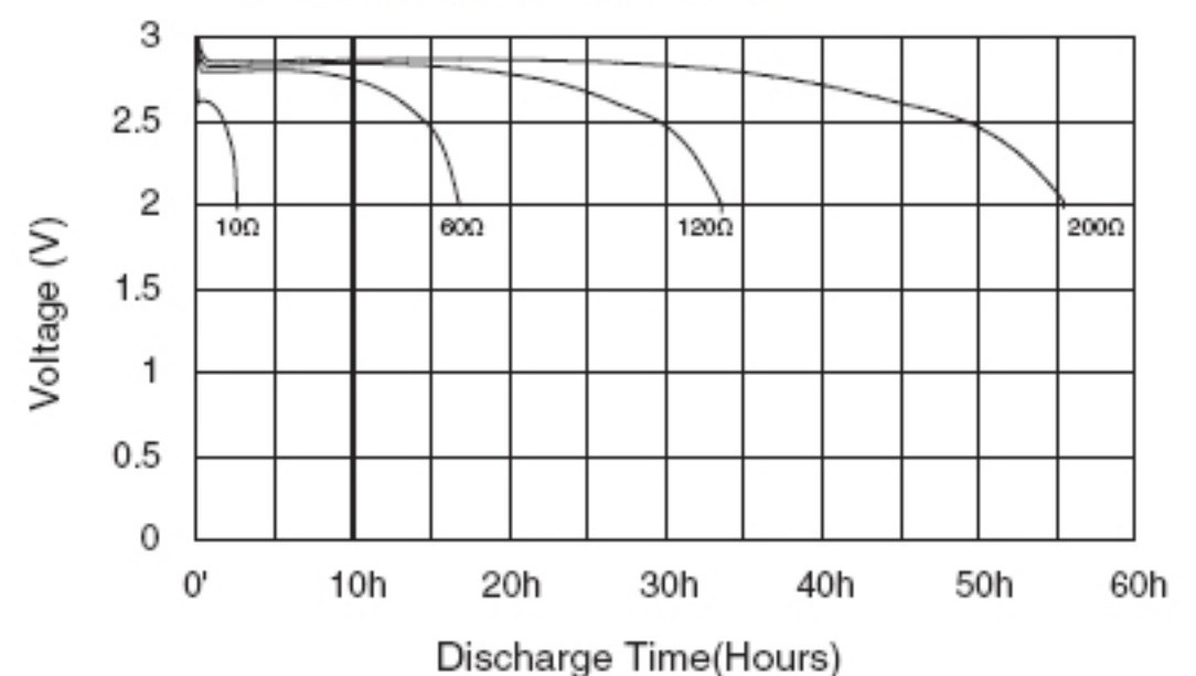
Continuous Discharge at 23^{\circ}\text{C}
