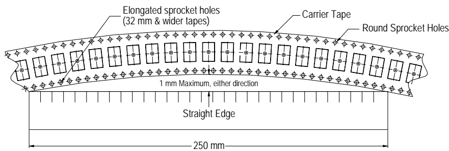
Figure 8 – Maximum Camber
