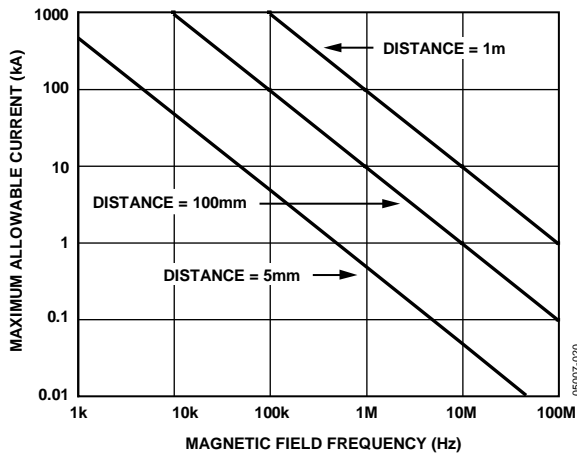
Figure 20. Maximum Allowable Current for Various Current-to-ADuM240x Spacings
