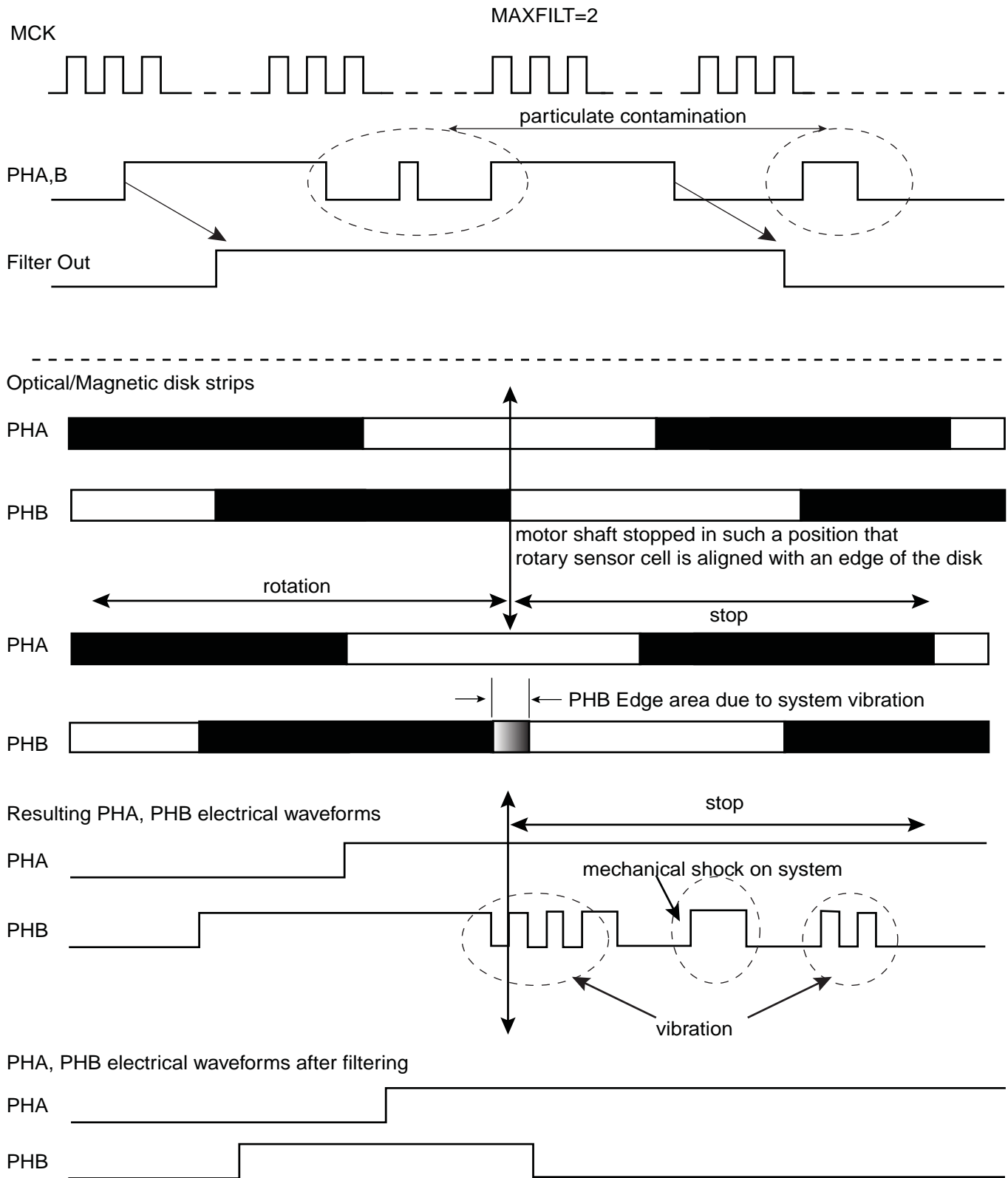
Figure 33-19. Filtering Examples
