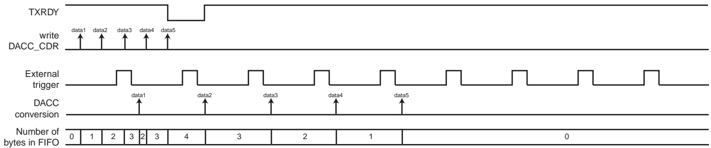
Figure 36-3. External trigger
