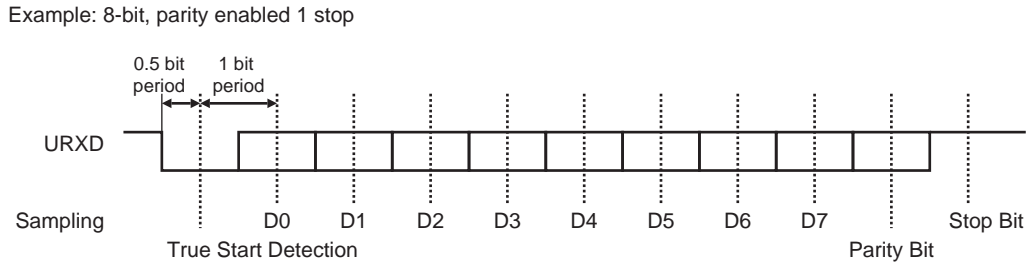
Figure 31-4. Character Reception
