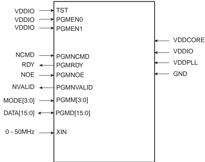
Figure 22-1. SAM4NxB/C Parallel Programming Interface
