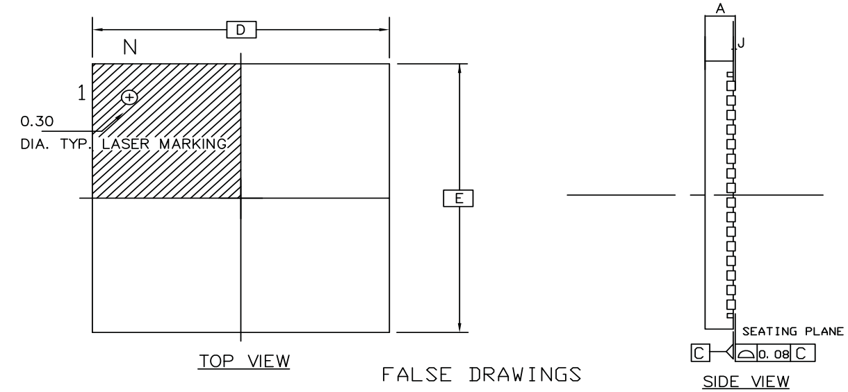
Figure 38-7. 48-pad QFN Package Drawing
