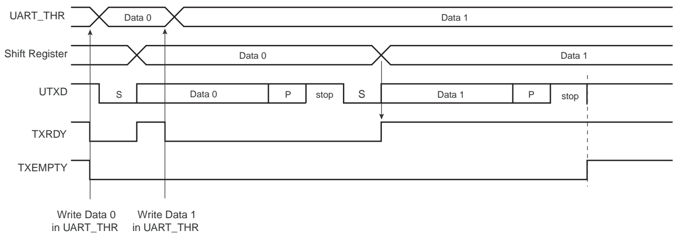
Figure 31-10. Transmitter Control
