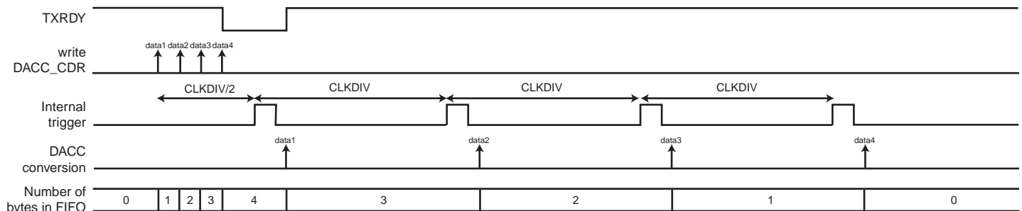
Figure 36-2. Internal trigger
