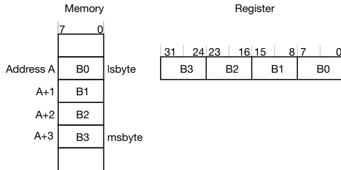
Figure 13-6. Little-endian Format
