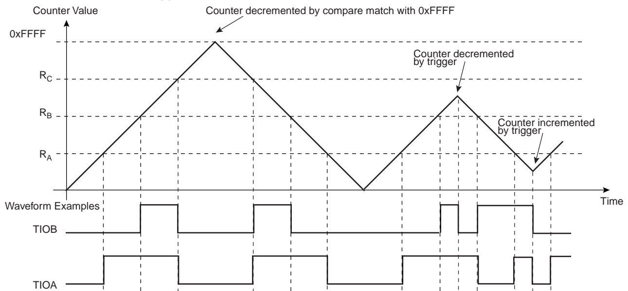
Figure 33-14. WAVSEL = 01 With Trigger
