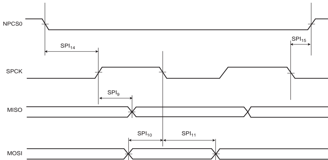
Figure 37-14. SPI Slave Mode with (CPOL = NCPHA = 0) or (CPOL = NCPHA = 1)
