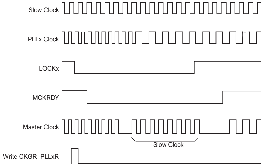
Figure 26-10. Change PLLx Programming
