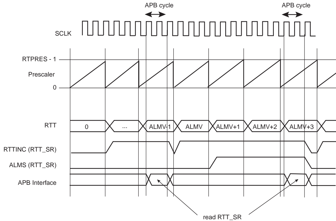
Figure 16-2. RTT Counting
