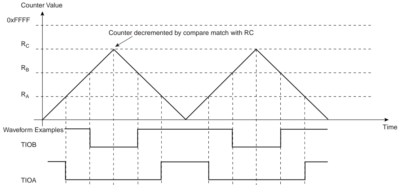
Figure 33-15. WAVSEL = 11 Without Trigger
