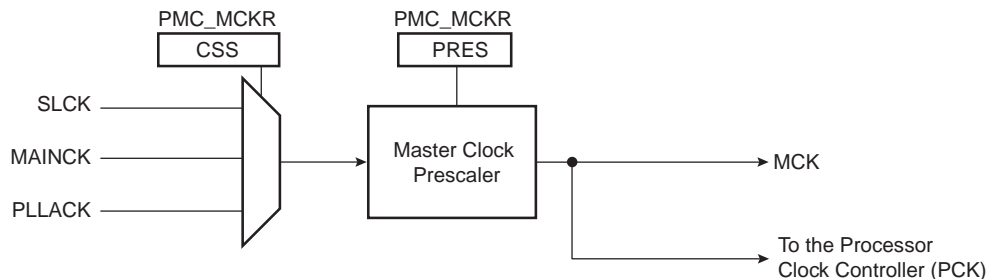
Figure 26-6. Master Clock Controller
