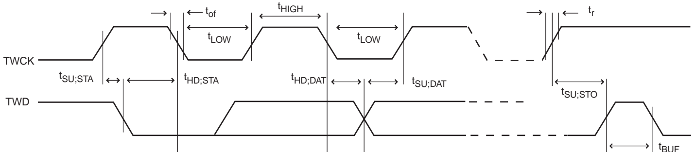
Figure 37-16.USART SPI Slave Mode (Mode 1 or 2)
