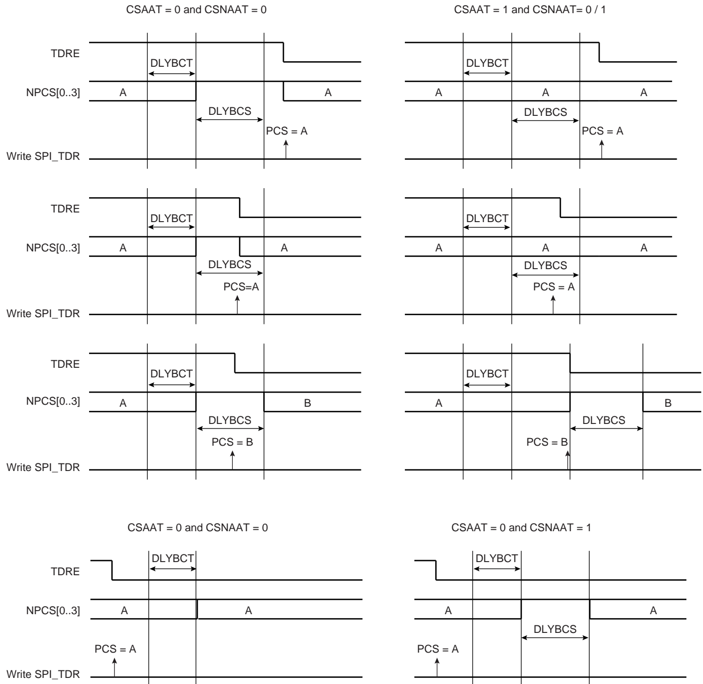
Figure 29-11. Peripheral Deselection
