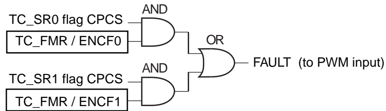
Figure 33-23. Fault Output Generation
