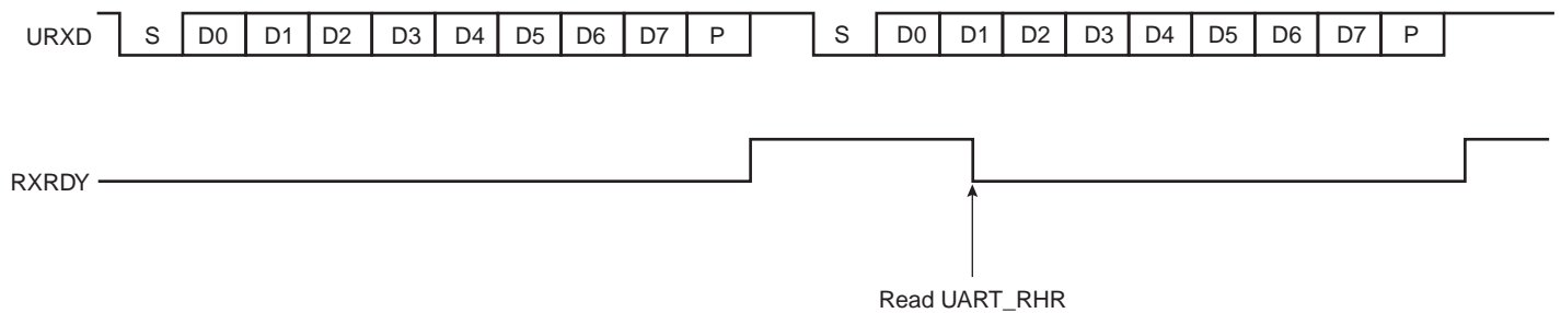
Figure 31-5. Receiver Ready
