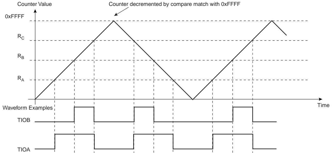
Figure 33-13. WAVSEL = 01 Without Trigger
