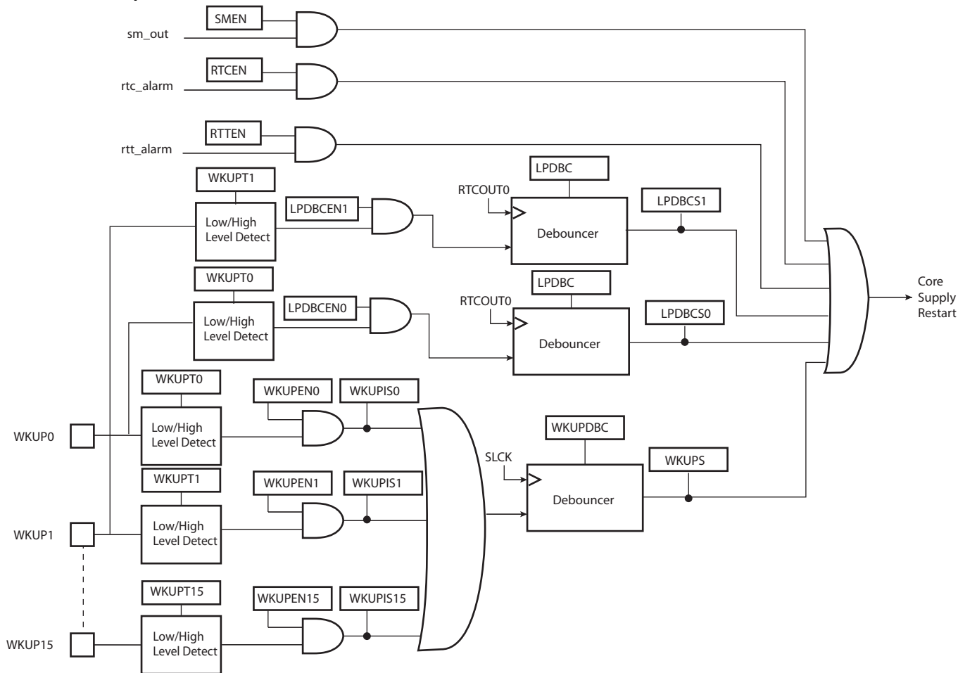
Figure 19-4. Wake-up Sources
