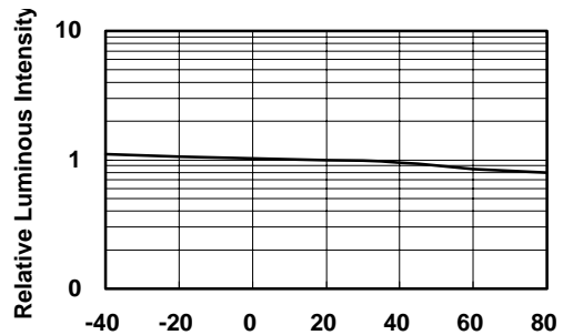
FIG4. LUMINOUS INTENSITY VS. AMBIENT TEMPERATURE
