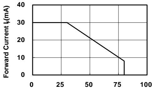
FIG3-27. FORWARD CURRENT VS. AMBIENT TEMPERATURE
