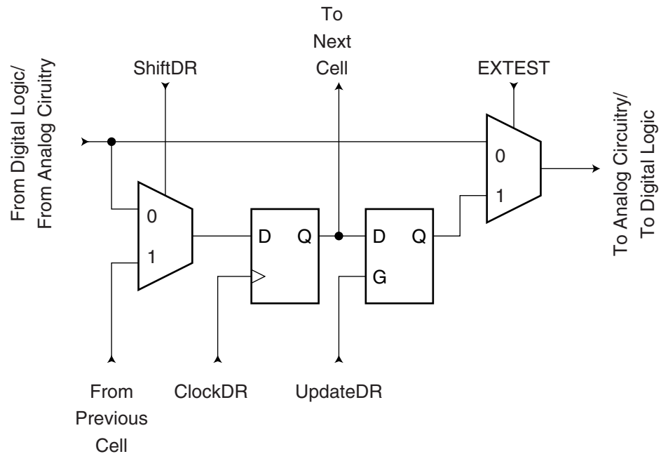
Figure 25-9. General Boundary-scan Cell used for Signals for Comparator and ADC
