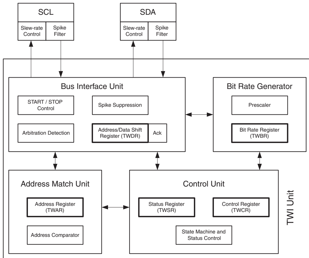
Figure 21-1. Overview of the TWI Module
