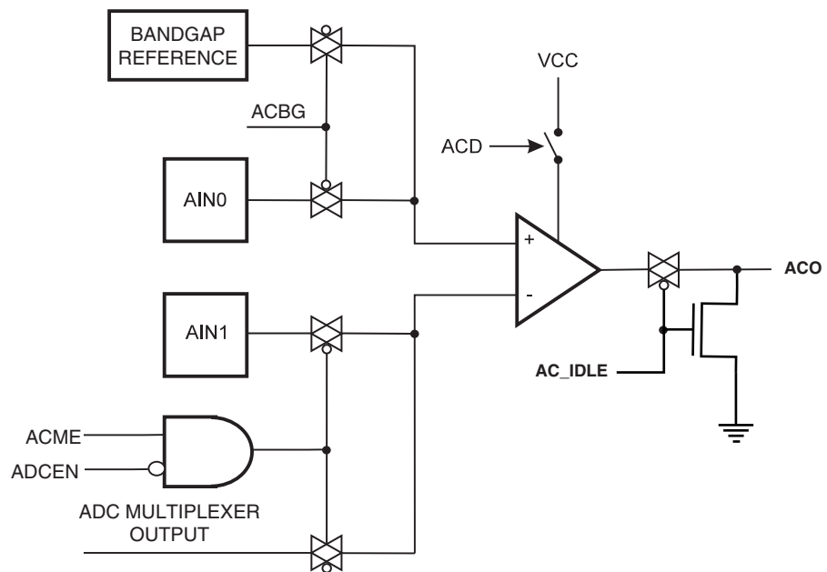
Figure 25-8. Analog Comparator
