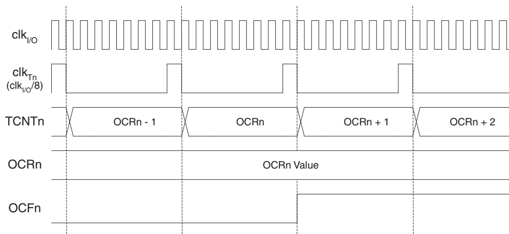
Figure 17-10. Timer/Counter Timing Diagram, Setting of OCF2, with Prescaler ( f_{clk\_I/O}/8 )
