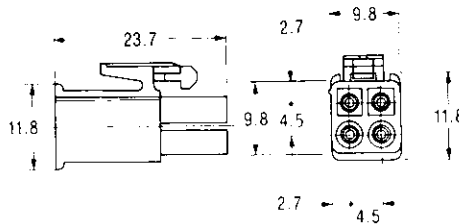
Plug (Reinforced Type)
