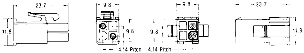
Plug
