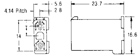
Cap (Free-Hanging)
