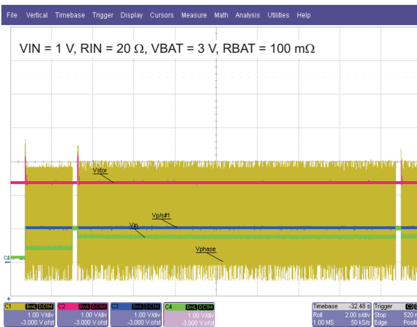
Figure 21. Example of Sampling Time for MPPT Operation
