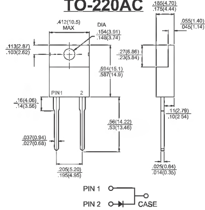
Dimensions in inches and (millimeters) Marking Diagram
