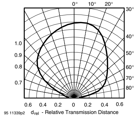
Figure 13. Vertical Directivity
