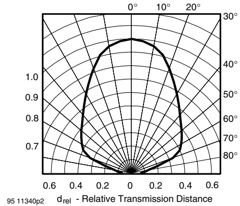
Figure 12. Horizontal Directivity
