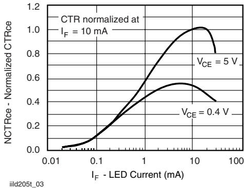
iiid205t_03 Figure 3. Normalized CTR_{ce} vs. Forward Current
