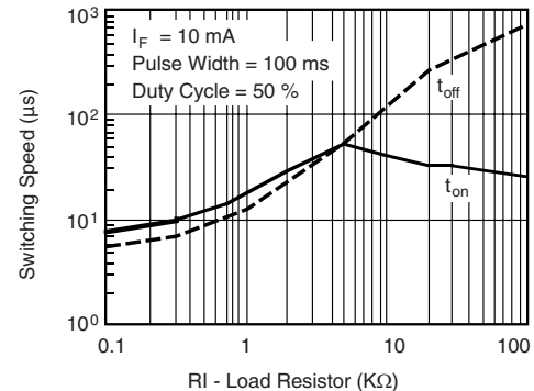
iiid205t_01 Figure 5. Switching Speed vs. Load Resistor
