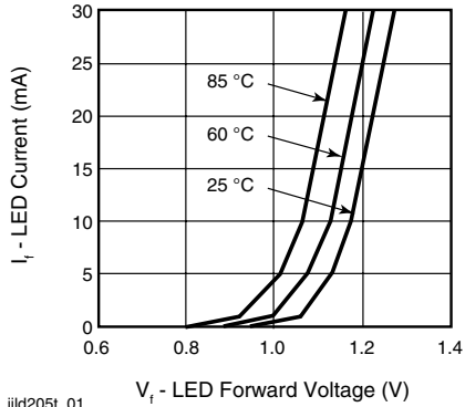
iiid205t_01 Figure 1. Forward Current vs. Forward Voltage
