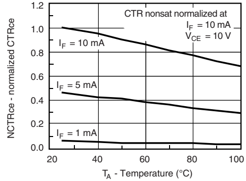
iiid205t_04 Figure 4. Current Transfer Ratio (normalized) vs. Ambient Temperature
