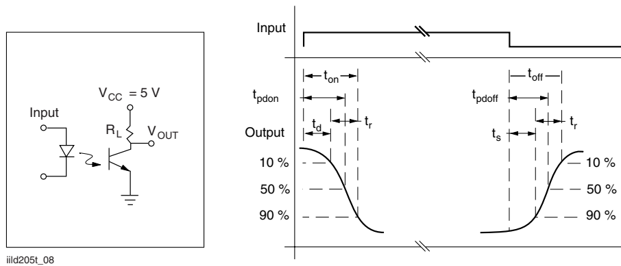
Figure 8. Switching Test Circuit
