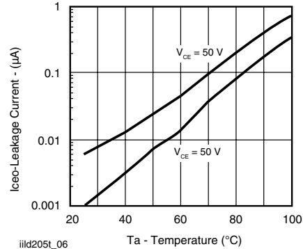
iiid205t_06 Figure 6. Collector Current vs. Ambient Temperature
