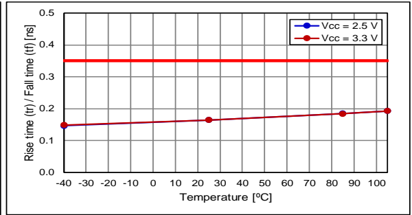
Fall Time
