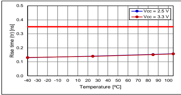
Rise Time
