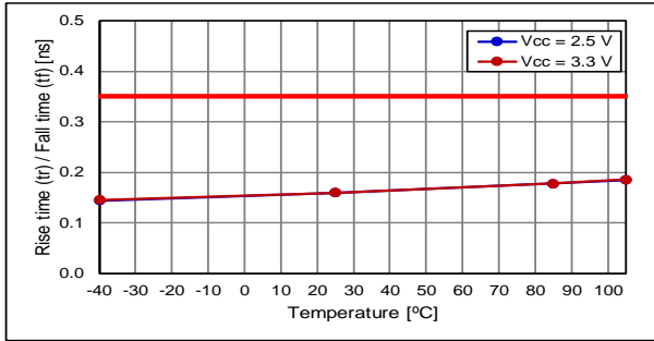
Rise Time
