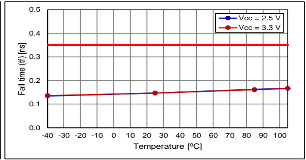
Fall Time
