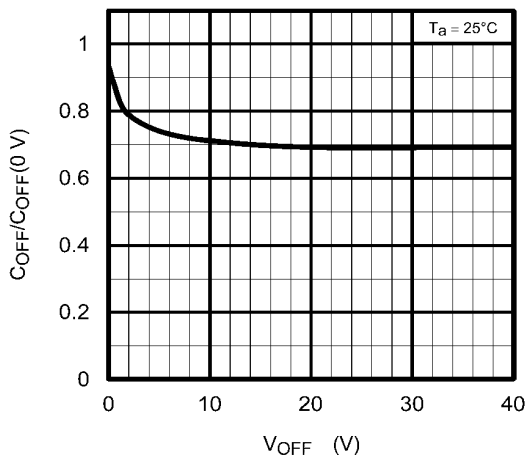
Fig. 12.11 C_{OFF}/C_{OFF(0V)} - V_{OFF}
