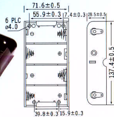
SN-14-2 / UM-1x4 FOR FOUR " D " CELL
