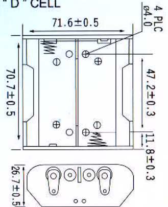
SN-12-1 / UM-1x2 FOR TWO " D " CELL
