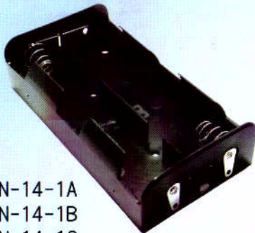
SN-14-1 / UM-1x4 FOR FOUR " D " CELL
