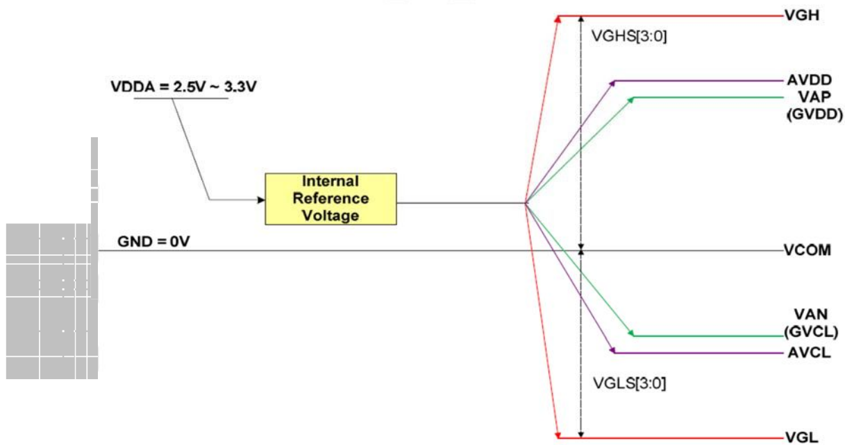
Fig.2 Voltage Generation
