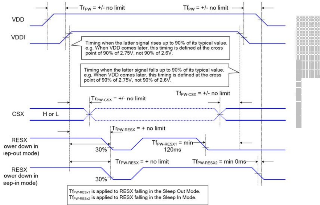
Fig.1 Power ON/OFF Sequence
