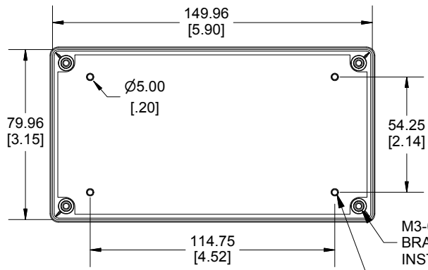
INSIDE BOX
