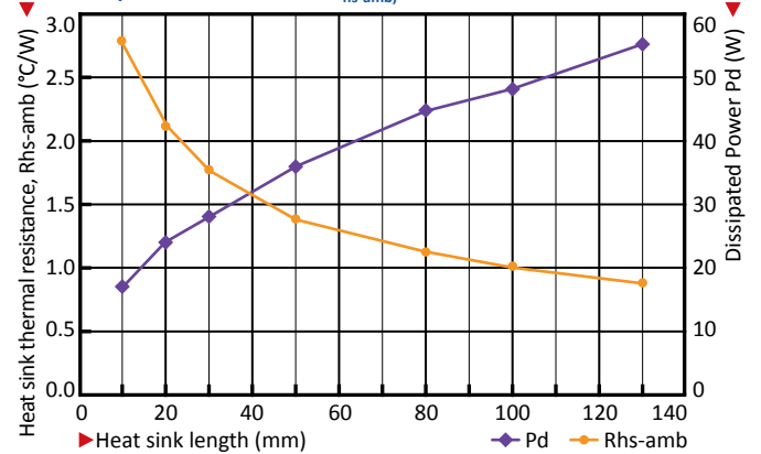
XSA-97 performance data at a heat sink to ambient temperature difference, \Delta T_{hs-amb} , of 50 ^{\circ}C
