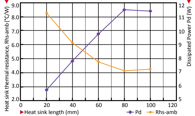
XSA-216 performance data at a heat sink to ambient temperature difference, ΔT hs-amb , of 50 °C
